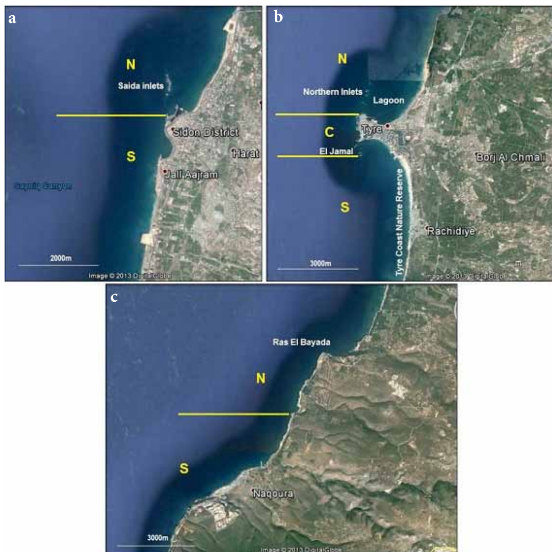
Figure 9. Studied areas (from North to South): Saida (a), Tyre (b) and Nakoura (c) (images from Google-Earth)
