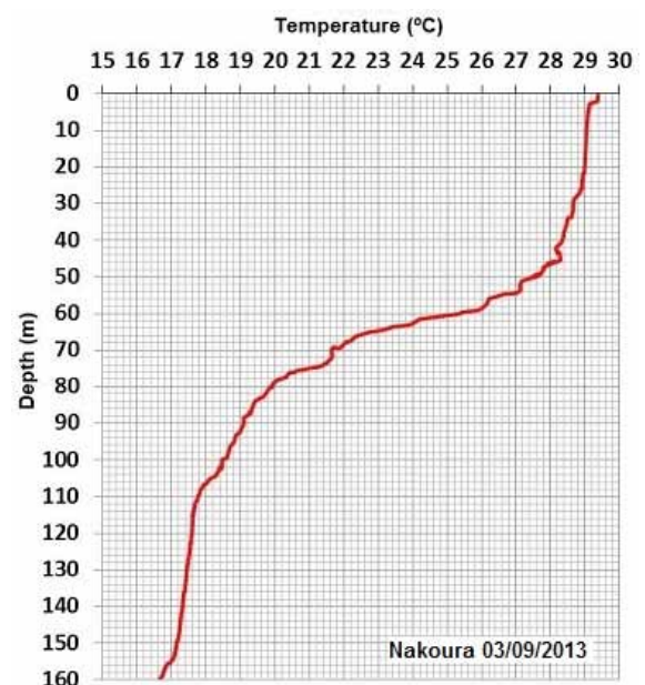
Figure 13. Temperature profiles in Nakoura and Kasmieh
