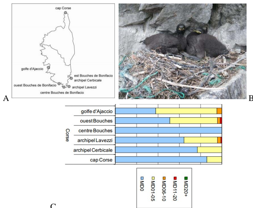
Figure 3: Percentage of nests containing marine litter and average number of bits of litter observed in the nests of Mediterranean shags ( Phalacrocorax aristotelis ) in Corsica (Work of the Bonifacio Reserve, the Corsican Conservatory of Natural Species, and IFREMER and Bretagne Vivante: Cadiou et al. , 2016). The results show the possibility of distinguishing the areas subject to human-origin impact from the areas least affected by pollution. (A) Sites of observations; (B) Nest of Mediterranean shag (credit B. Cadiou) occupied by two fledglings; the marine litter, here mainly cordage, has been used just like natural materials to build the nest; (C) Number of bits of litter per nest (N=556 sampled nests). Each horizontal histogram represents for each site 100% of nests and each colour the percentage of nests (vertical graduation = 20%) with a variable number of bits of litter (MD) (0.1 to 5.6 to 10.11 to 20 and over 20).
