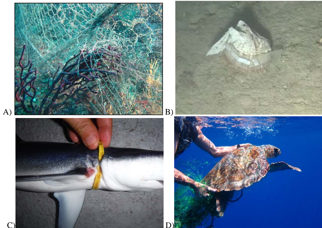
Figure 2: Strangling/entanglement of marine organisms. (A) A Paramuricea sp. gorgonian entangled in a ghost fishing net (credit M. Matiddi, as per Werner et al., 2017); (B) An urchin covered with two plastic sheets (credit F. Galgani, unpublished); (C) A Prionace glauca shark strangled by a plastic ring (credit M. P. Salinas, as per Colmenero et al., 2017); (D) Turtle entangled in a lost net (credit Alnitak)
