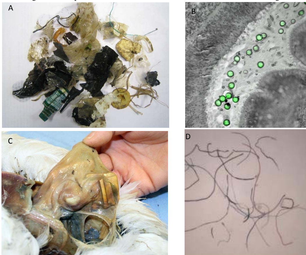
Figure 1: Marine litter ingested by Mediterranean marine organisms. (A) Marine litter excreted by a turtle in a rescue center in the French Mediterranean (species Caretta caretta , rescue center CESTMed, credit CESTMed). (B) Micro-plastics highlighted by fluorescence during an experimental study of the (in vitro) transit of micro-plastics in the digestive gland of an oyster ( Crassostrea gigas ) (credit A. Huvet, IFREMER). (C) Marine litter ingested by a North Sea northern fulmar ( Fulmaris glacialis , credit J. Van Franeker, IMARES). (D) Fibres ingested by an individual of the fish species Boops boops sampled in the Balearic Islands (credit COB-IEO/Spain).
